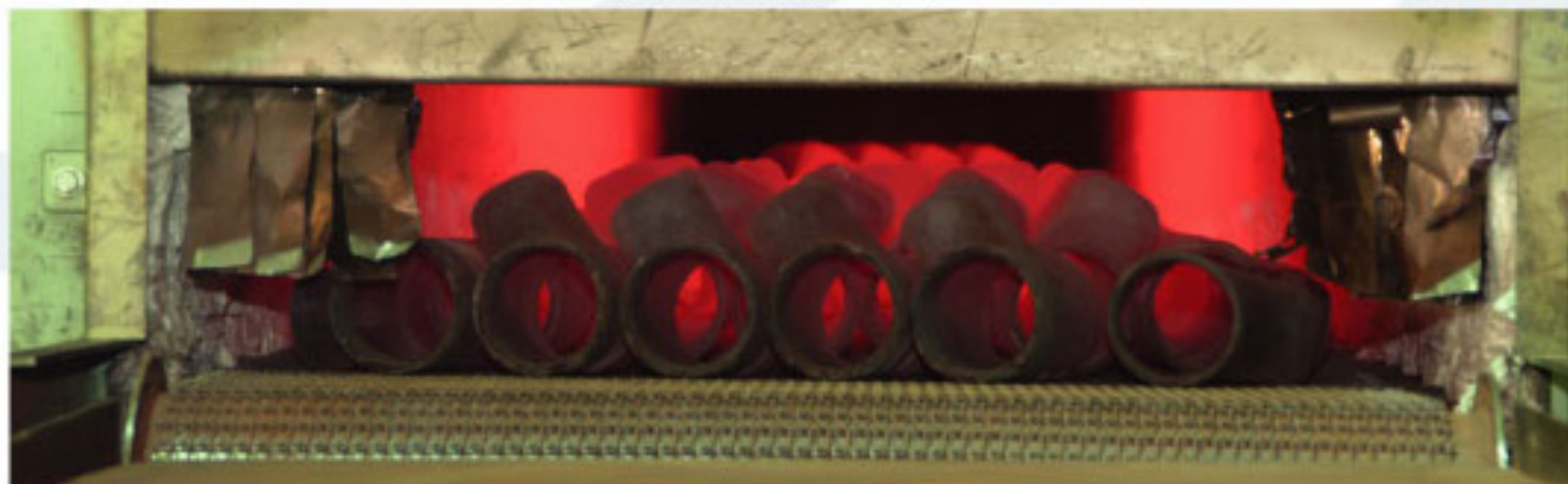
Normalising Furnace
